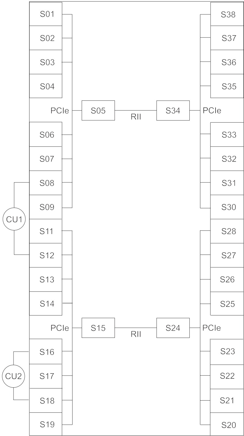
Figure 1. I/O channel path configuration for a representative PCIe I/O drawer in a 2817, 2818 and 2827 model
