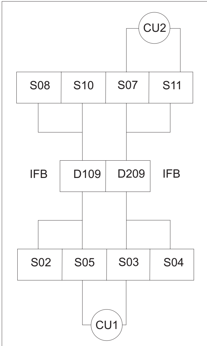
Figure 3. I/O channel path configuration for a representative I/O drawer in a 2828, 2817, 2818, and 2827 model
